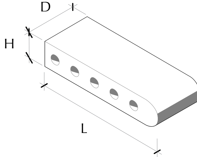
Pool Coping Dimensions, Weights, and Coverage
