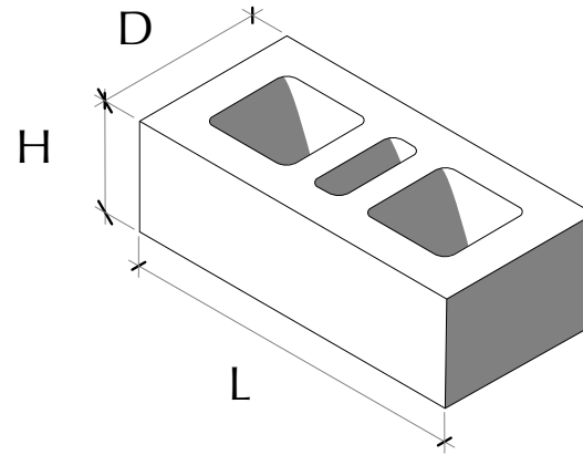
Atlas® Brick Dimensions, Weights, and Coverage
